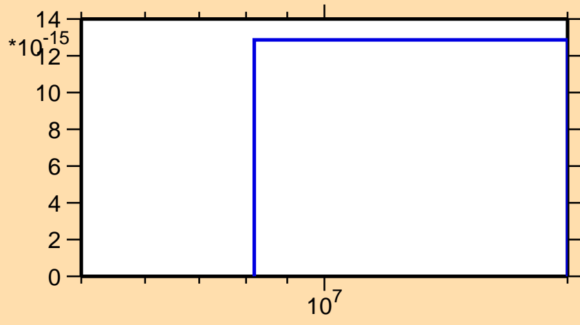
\sigma vs. E for ^{147}\text{Eu}(n,\text{pt})
