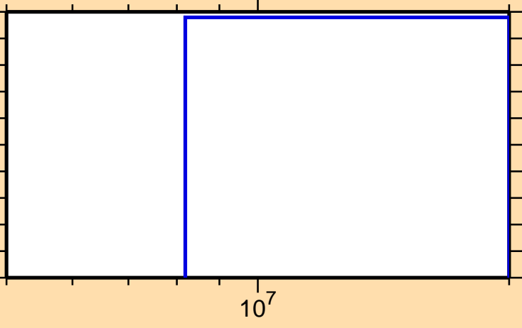
\sigma vs. E for ^{147}\text{Eu}(n,2n\alpha)
