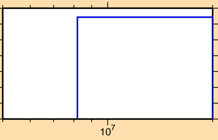
\sigma vs. E for ^{147}\text{Eu}(n,\text{pt})
