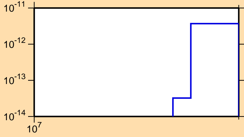
\sigma vs. E for ^{148}\text{Eu}(n,\text{pd})
