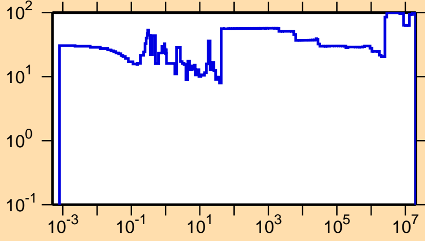
\Delta\sigma/\sigma vs. E for ^{148}\text{Eu}(n,\gamma)
