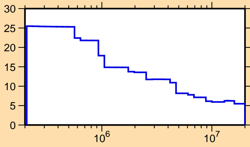
\Delta\sigma/\sigma vs. E for ^{148}\text{Eu}(n,\text{nonel.})
