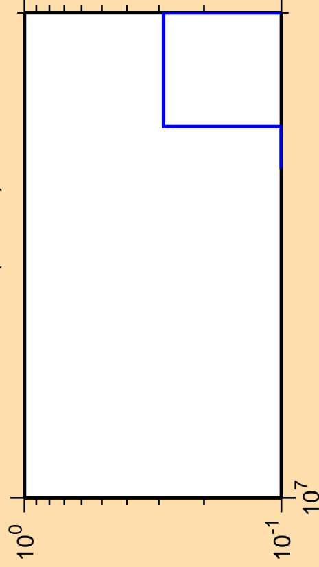
\Delta\sigma/\sigma vs. E for ^{148}\text{Eu} (mt 11)
