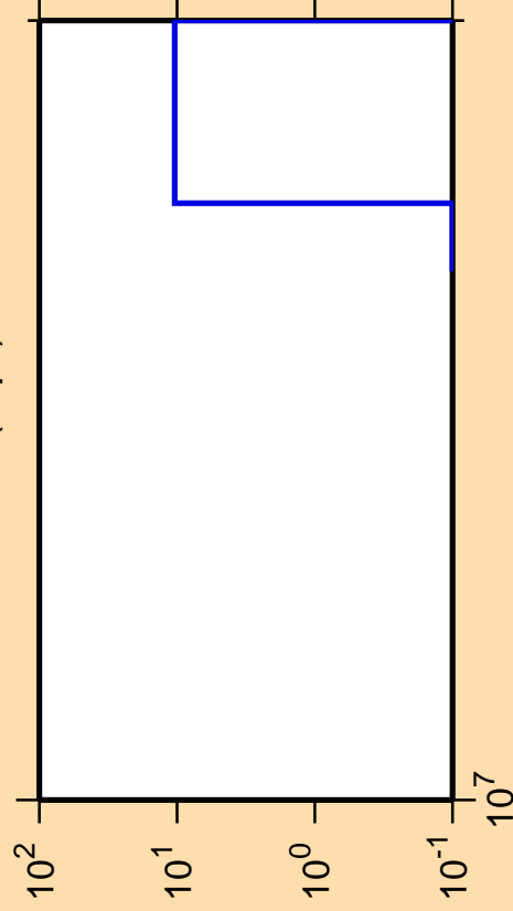
\Delta\sigma/\sigma vs. E for ^{148}\text{Eu}(n,pt)
