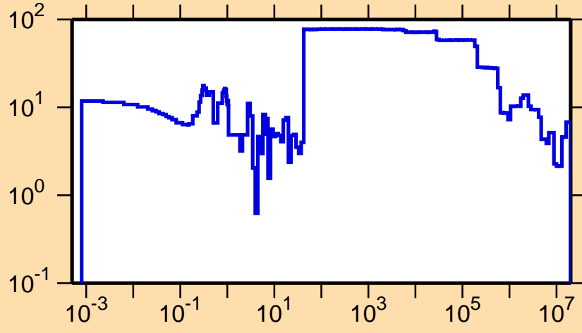
\Delta\sigma/\sigma vs. E for ^{148}\text{Eu}(n,\text{tot.})
