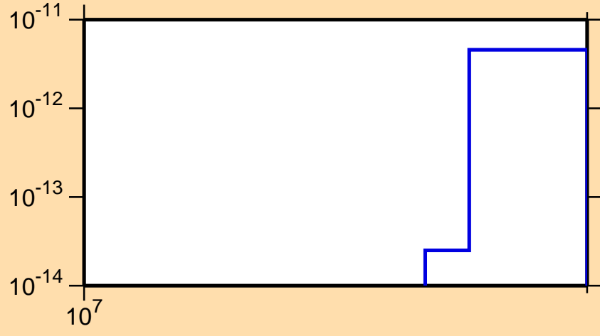
\sigma vs. E for ^{148}\text{Eu}(n,pt)
