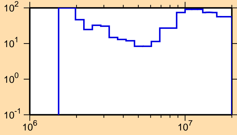
\Delta\sigma/\sigma vs. E for ^{148}\text{Eu}(n,n\text{cont.})
