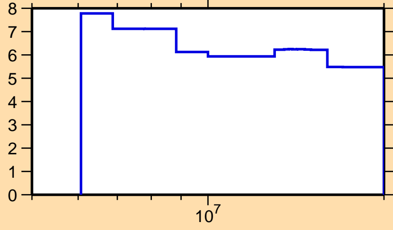
\Delta\sigma/\sigma vs. E for ^{148}\text{Eu}(n,\text{nonel.})
