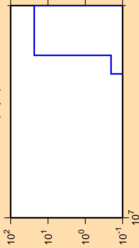
\Delta\sigma/\sigma vs. E for ^{148}\text{Eu}(n,\text{pd})
