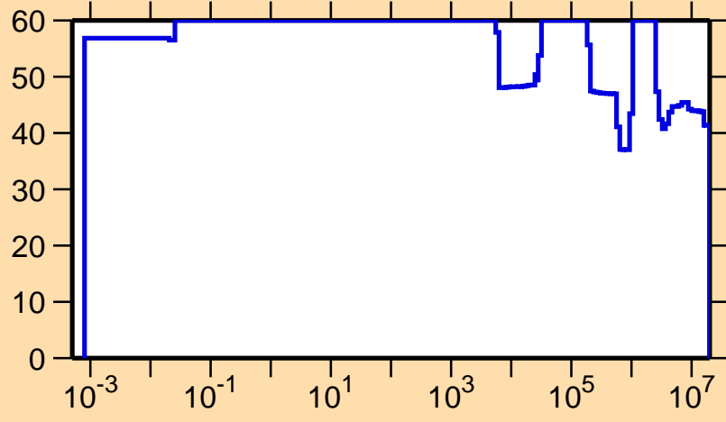
\Delta\sigma/\sigma vs. E for ^{148}\text{Eu}(n,p)
