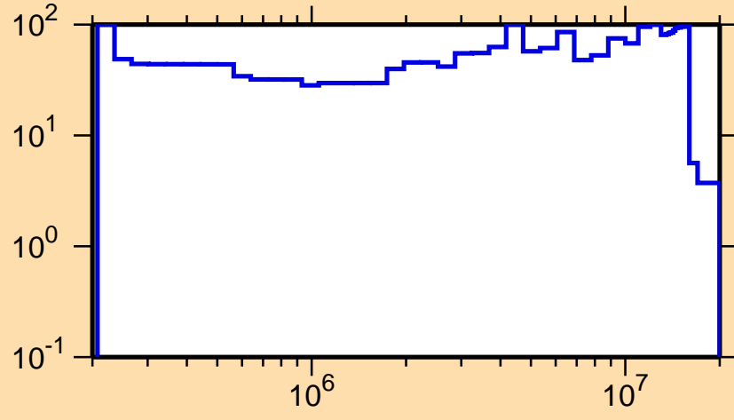
\Delta\sigma/\sigma vs. E for ^{148}\text{Eu}(n,n_1)
