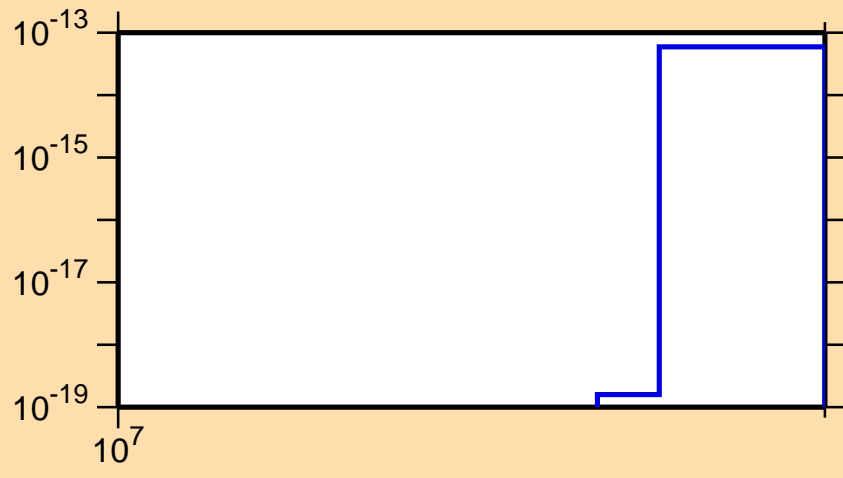
\sigma vs. E for ^{148}\text{Eu} (mt 11)
