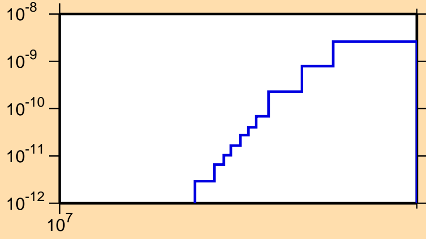
\sigma vs. E for ^{148}\text{Eu}(\text{mt117})
