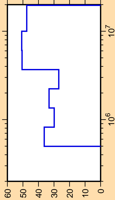
\Delta\sigma/\sigma vs. E for ^{148}\text{Eu}(n,n_3)
