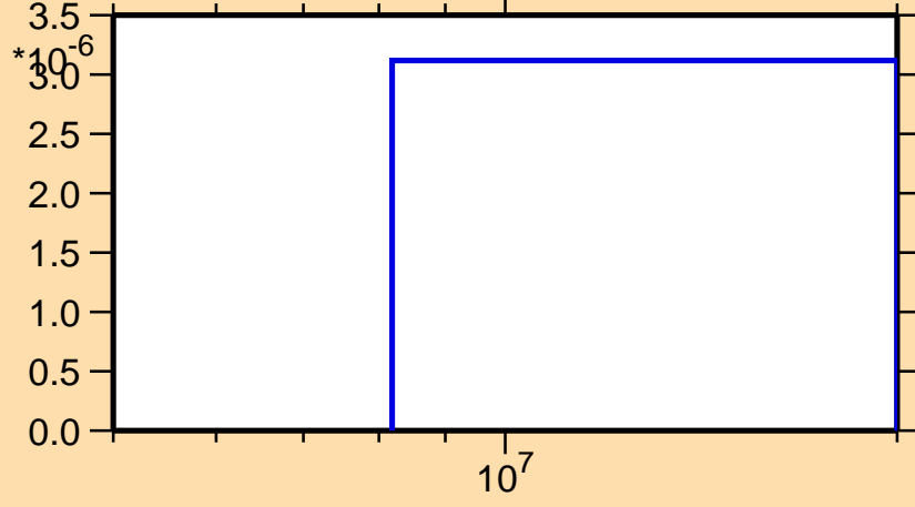
\sigma vs. E for ^{148}\text{Eu}(n,nd)
