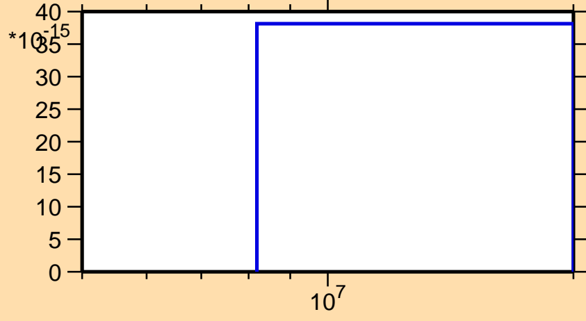
\sigma vs. E for ^{148}\text{Eu}(n,pt)
