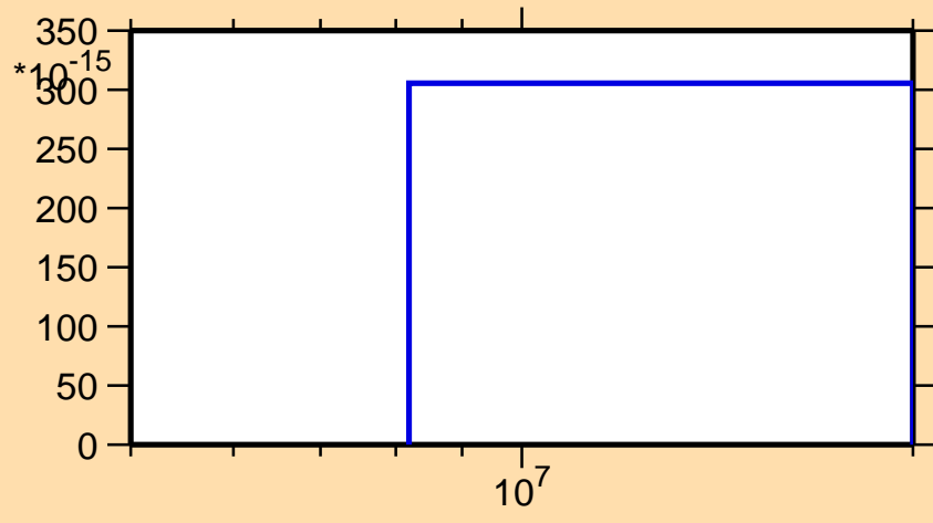
\sigma vs. E for ^{148}\text{Eu}(\text{mt } 34)
