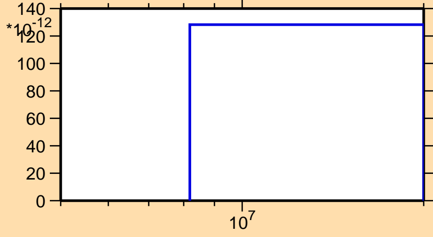
\sigma vs. E for ^{148}\text{Eu} (mt 45)
