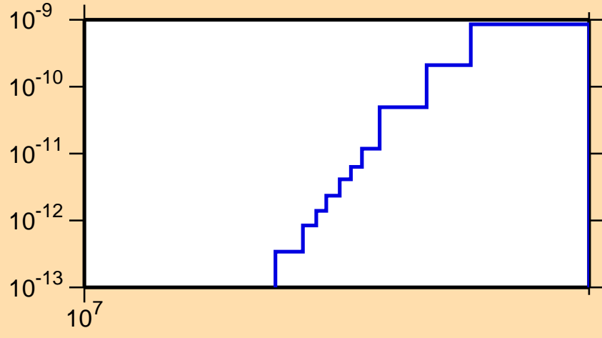
\sigma vs. E for ^{149}\text{Eu}(\text{mt117})
