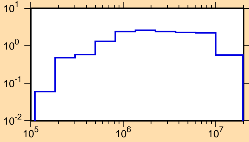
\sigma vs. E for ^{149}\text{Eu}(n,\text{inel.})
