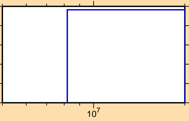
\sigma vs. E for ^{149}\text{Eu}(n,2n\alpha)
