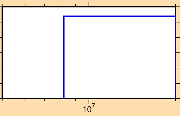
\sigma vs. E for ^{149}\text{Eu}(n,3n)
