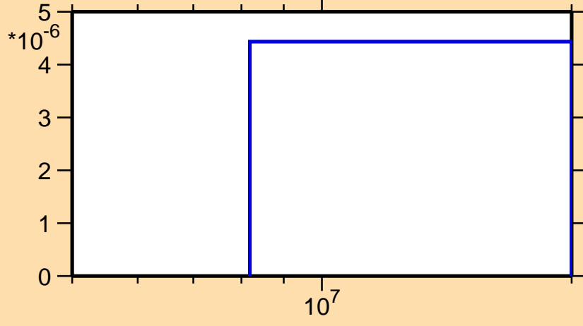
\sigma vs. E for ^{150}\text{Eu}(n,2n\alpha)
