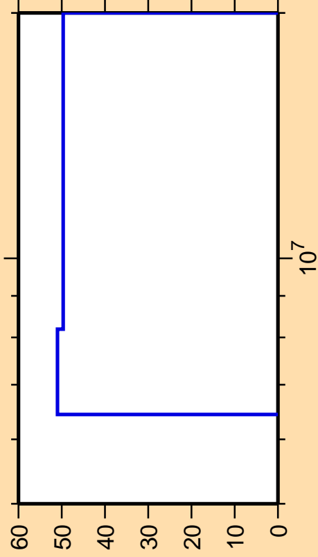
\Delta\sigma/\sigma vs. E for ^{150}\text{Eu}(n,p)
