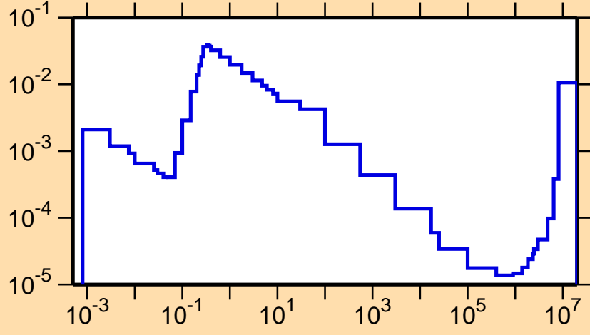
\sigma vs. E for ^{150}\text{Eu}(n,\alpha)
