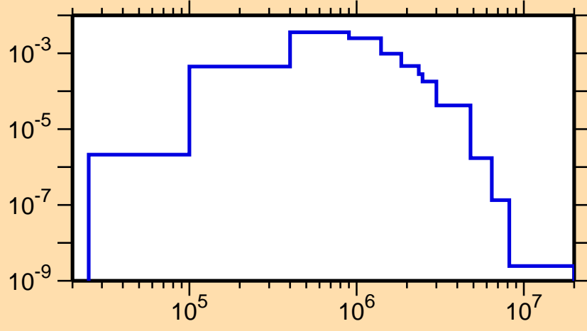
\sigma vs. E for ^{150}\text{Eu}(n,n_1)
