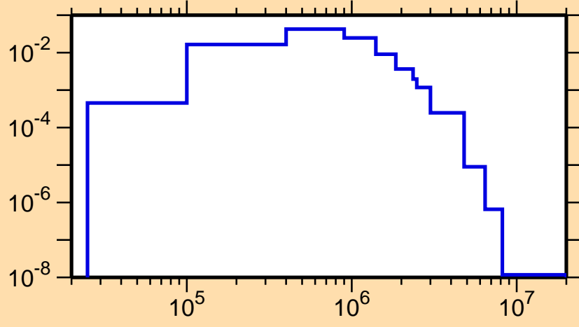
\sigma vs. E for ^{150}\text{Eu}(n,n_3)
