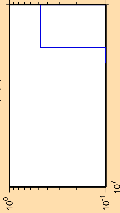
\Delta\sigma/\sigma vs. E for ^{150}\text{Eu}(n,\text{pt})
