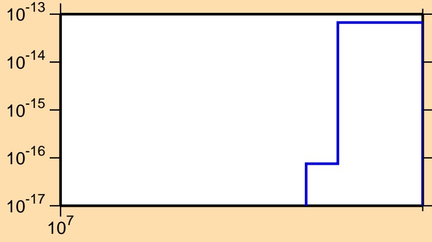
\sigma vs. E for ^{150}\text{Eu}(n,\text{pt})
