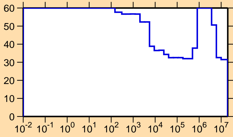
\Delta\sigma/\sigma vs. E for ^{150}\text{Eu}(n,p)
