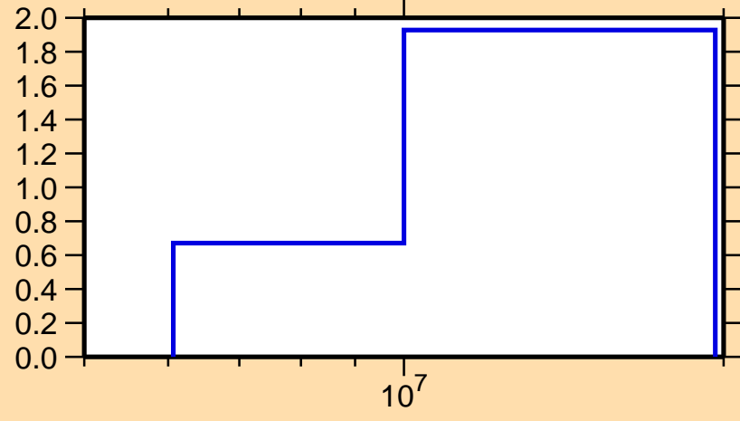
\sigma vs. E for ^{150}\text{Eu}(n,2n)
