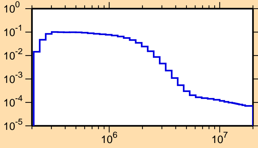
\sigma vs. E for ^{151}\text{Eu}(n,n_3)
