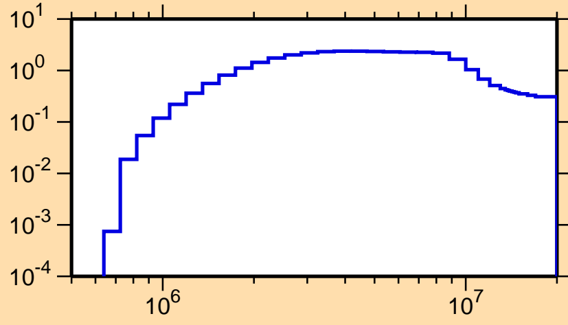
\sigma vs. E for ^{151}\text{Eu}(n,n\text{cont.})
