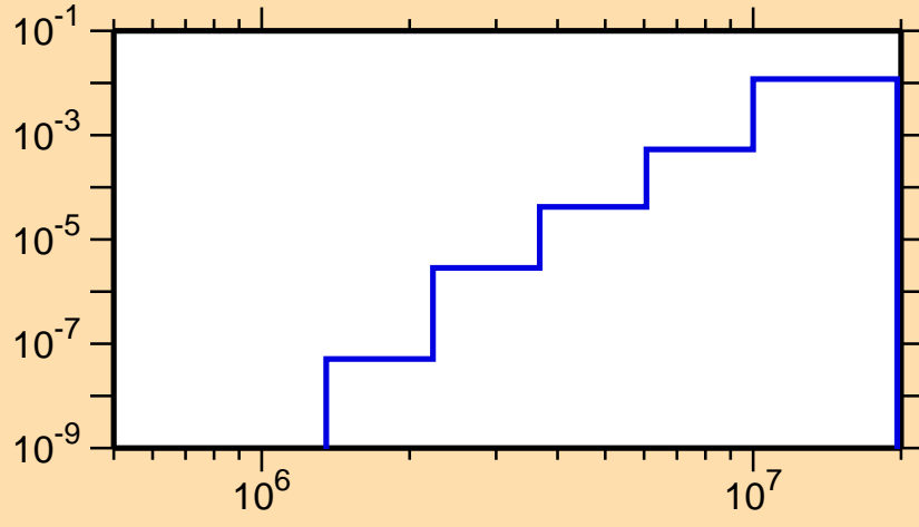
\sigma vs. E for ^{151}\text{Eu}(n,p)
