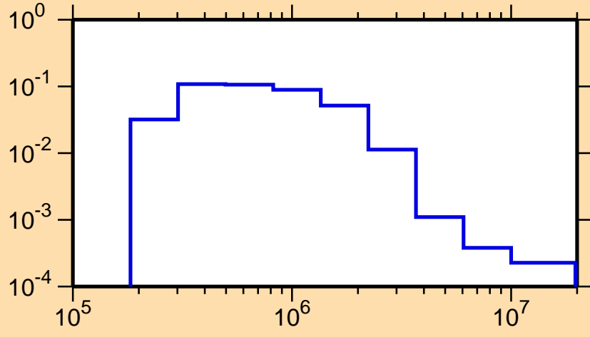
\sigma vs. E for ^{151}\text{Eu}(n,n_4)
