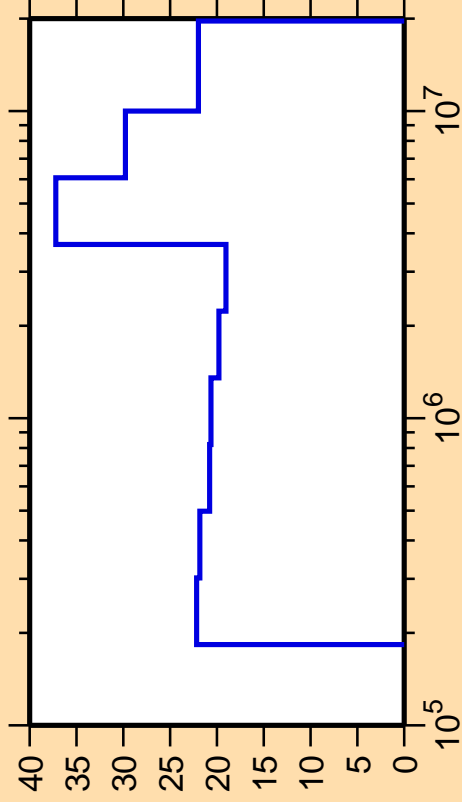
\Delta\sigma/\sigma vs. E for ^{151}\text{Eu}(n,n_4)
