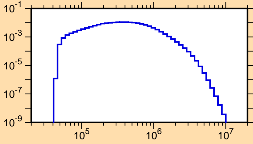
\sigma vs. E for ^{152}\text{Eu}(n,n_1)
