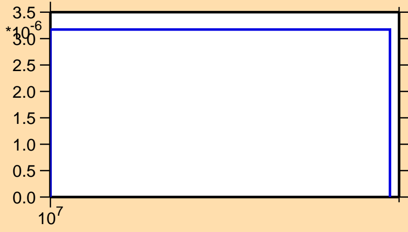
\sigma vs. E for ^{152}\text{Eu}(n,\text{nd})
