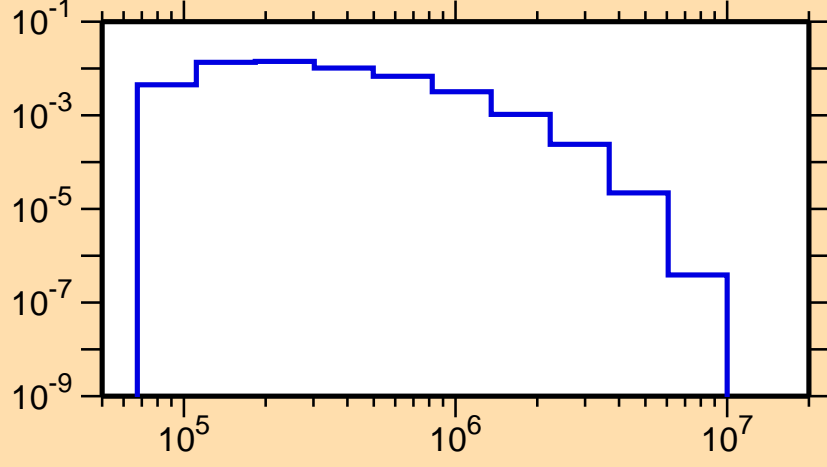
\sigma vs. E for ^{152}\text{Eu}(n,n_4)
