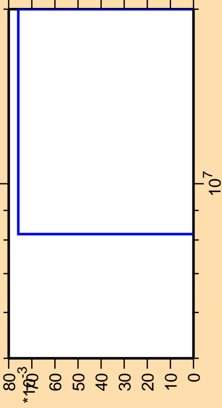
\Delta\sigma/\sigma vs. E for ^{152}\text{Eu}(\text{mt117})
