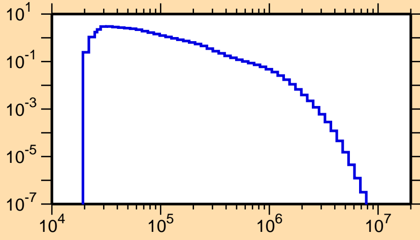
\sigma vs. E for ^{152}\text{Eu}(n,n_2)
