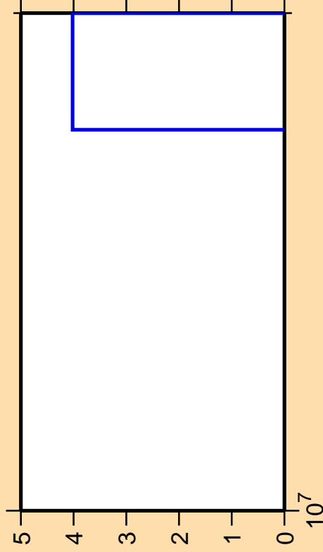
\Delta\sigma/\sigma vs. E for ^{152}\text{Eu} (mt 11)
