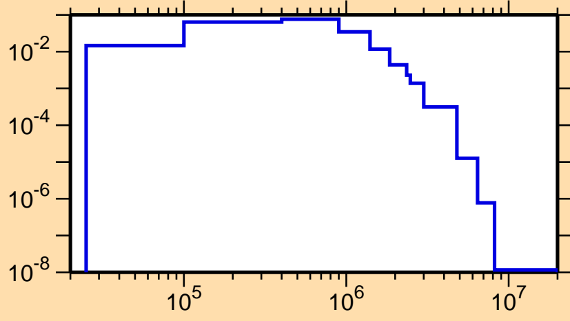
\sigma vs. E for ^{152}\text{Eu}(n,n_3)
