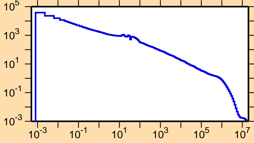
\sigma vs. E for ^{152}\text{Eu}(n,\gamma)
