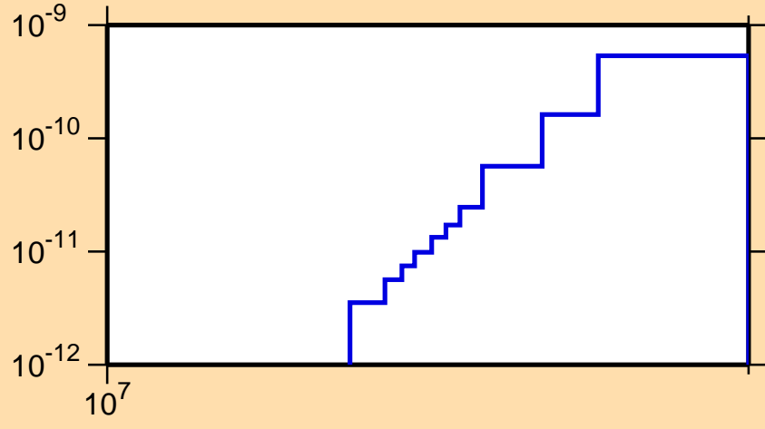
\sigma vs. E for ^{152}\text{Eu}(n,p\alpha)
