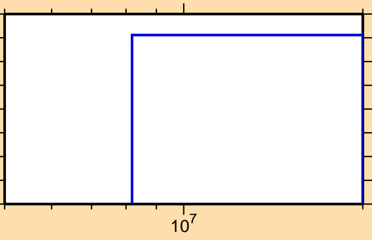
\sigma vs. E for ^{152}\text{Eu}(n,3n\alpha)
