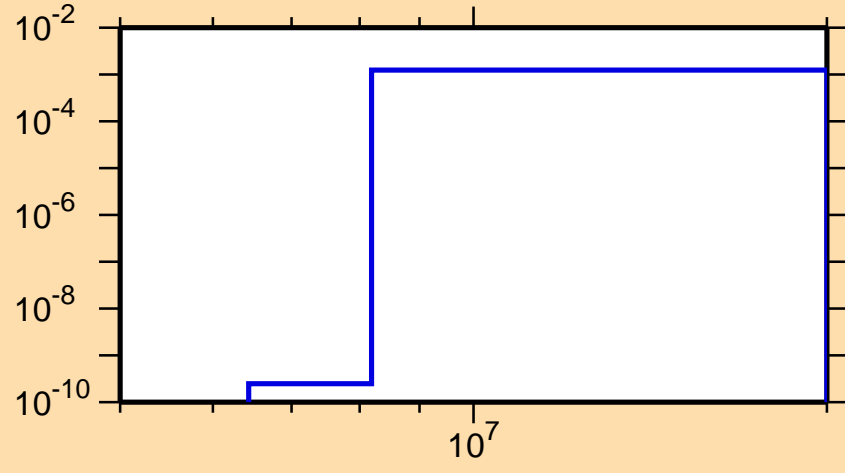
\sigma vs. E for ^{152}\text{Eu}(n,np)
