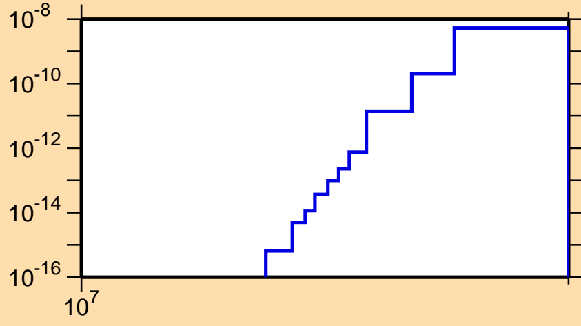
\sigma vs. E for ^{153}\text{Eu}(n,\text{He3})
