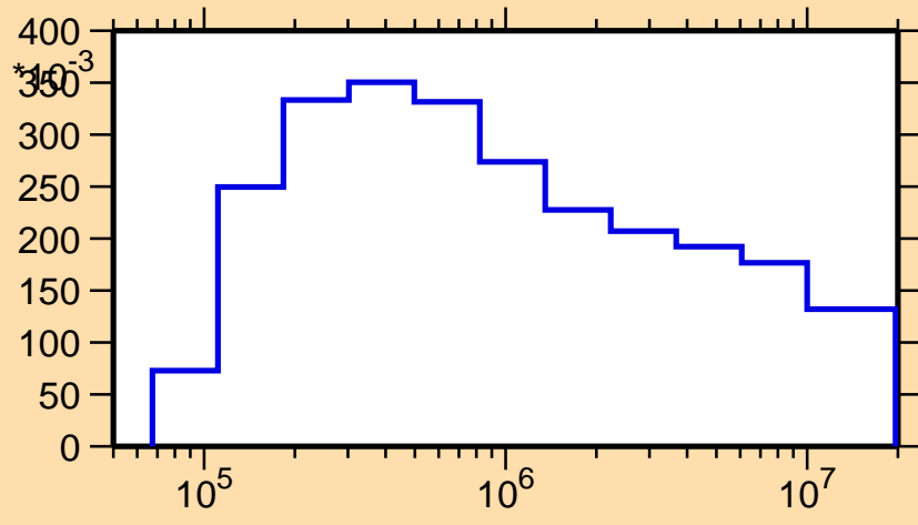
\sigma vs. E for ^{153}\text{Eu}(n,n_1)
