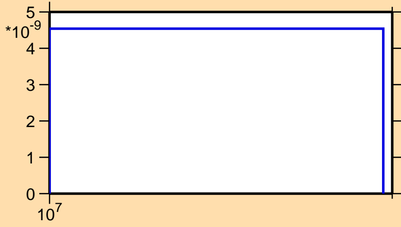
\sigma vs. E for ^{153}\text{Eu}(n,2n\alpha)
