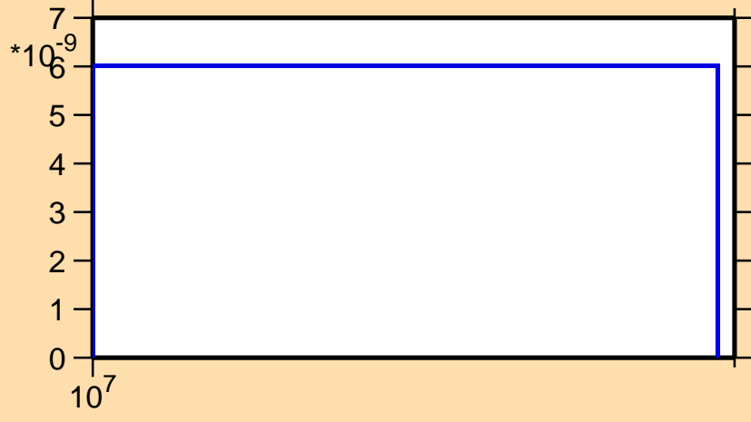
\sigma vs. E for ^{153}\text{Eu}(n,2np)
