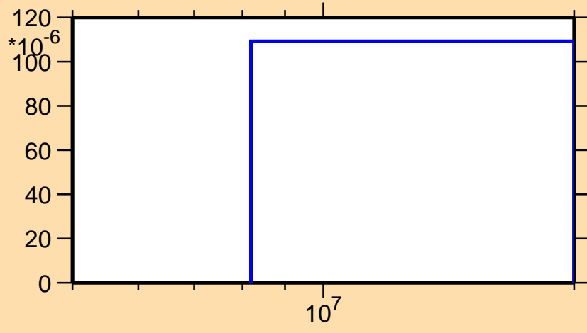
\sigma vs. E for ^{153}\text{Eu}(n,t)
