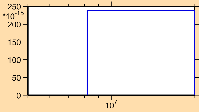
\sigma vs. E for ^{153}\text{Eu}(n,p\alpha)
