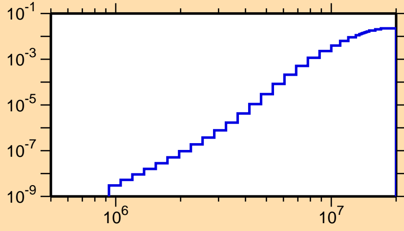
\sigma vs. E for ^{154}\text{Eu}(n,p)
