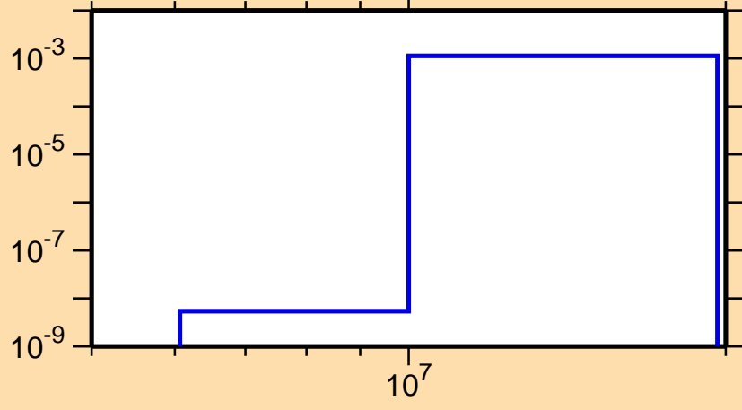
\sigma vs. E for ^{154}\text{Eu}(n,np)
