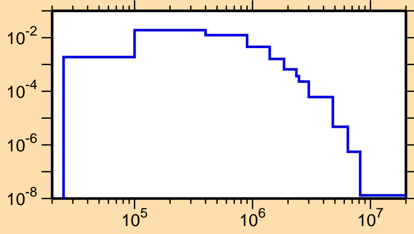
\sigma vs. E for ^{154}\text{Eu}(n,n_2)
