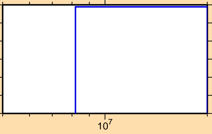
\sigma vs. E for ^{154}\text{Eu}(n,nd)
