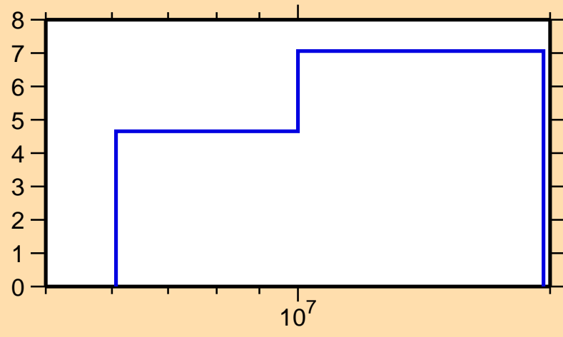
\Delta\sigma/\sigma vs. E for ^{154}\text{Eu}(n,\text{el.})
