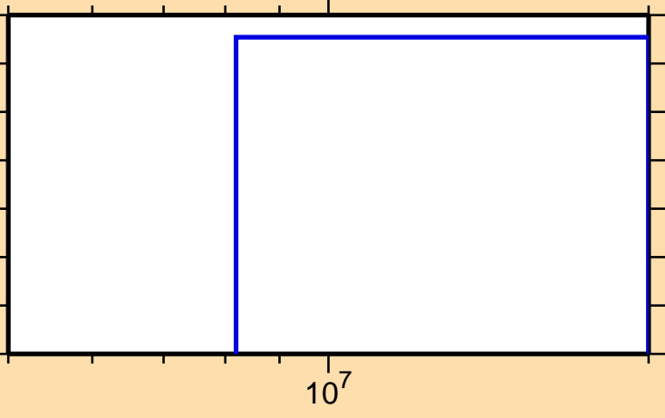
\sigma vs. E for ^{154}\text{Eu}(n,nt)
