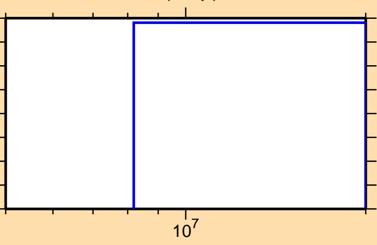
\sigma vs. E for ^{154}\text{Eu}(n,np)
