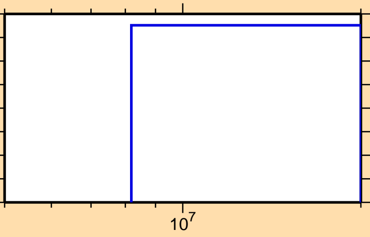
\sigma vs. E for ^{154}\text{Eu}(n,3n)
