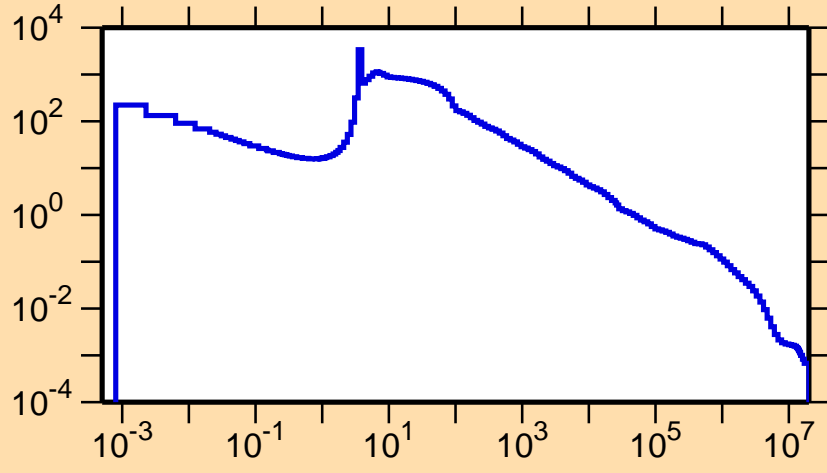
\sigma vs. E for ^{156}\text{Eu}(n,\gamma)
