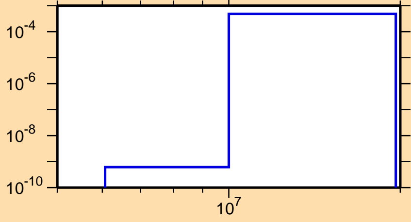
\sigma vs. E for ^{156}\text{Eu}(n,d)
