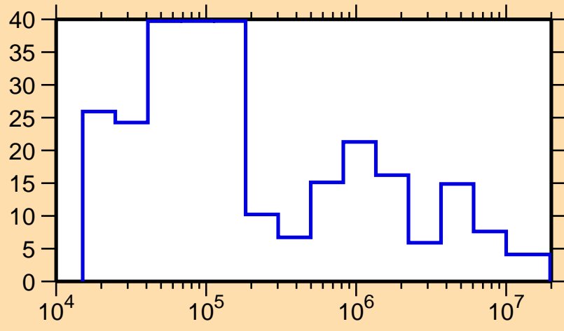
\Delta\sigma/\sigma vs. E for ^{156}\text{Eu}(n,\text{tot.})
