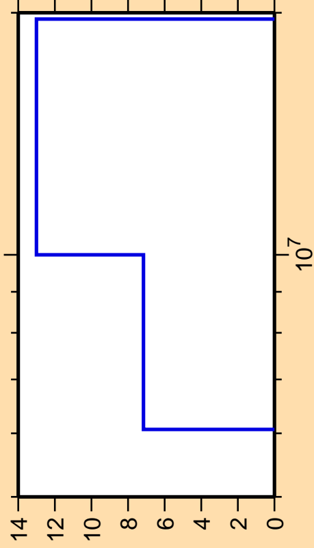
\Delta\sigma/\sigma vs. E for ^{156}\text{Eu}(n,2n)
