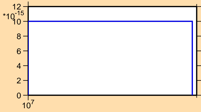
\sigma vs. E for ^{156}\text{Eu}(n,p\alpha)
