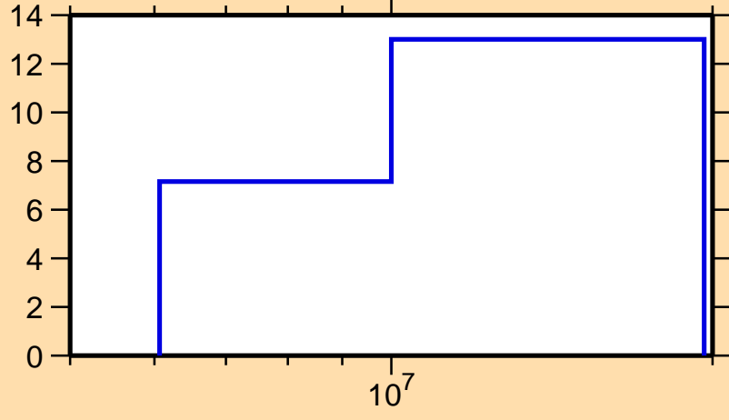
\Delta\sigma/\sigma vs. E for ^{156}\text{Eu}(n,2n)
