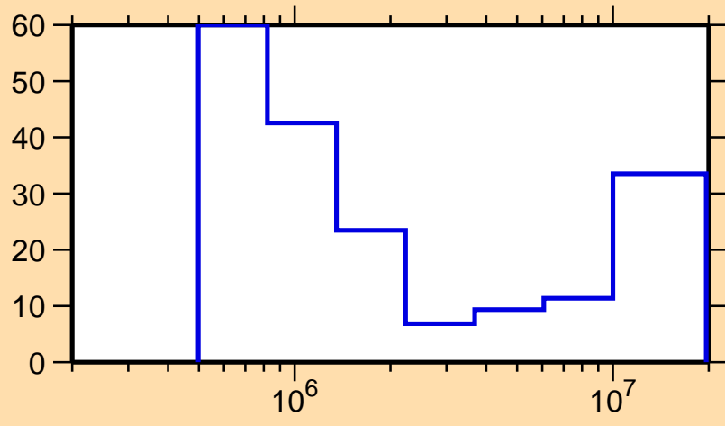
\Delta\sigma/\sigma vs. E for ^{156}\text{Eu}(n,n\text{cont.})
