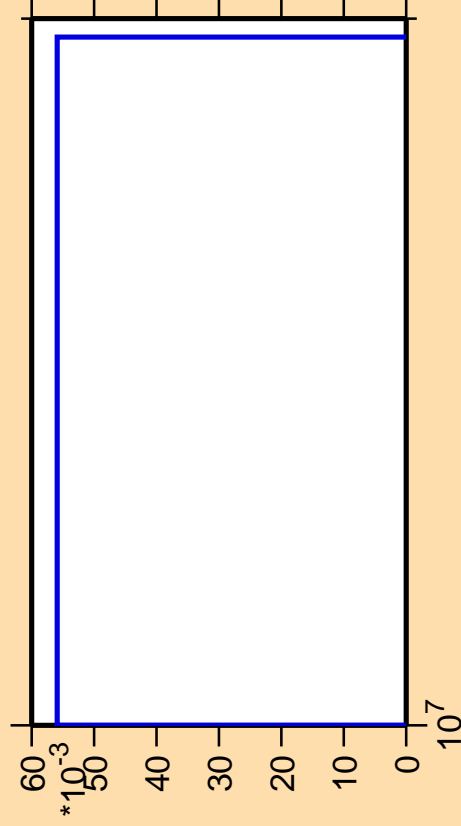
\Delta\sigma/\sigma vs. E for ^{156}\text{Eu}(n,p\alpha)
