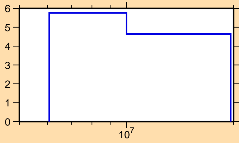
\Delta\sigma/\sigma vs. E for ^{156}\text{Eu}(n,\text{nonel.})
