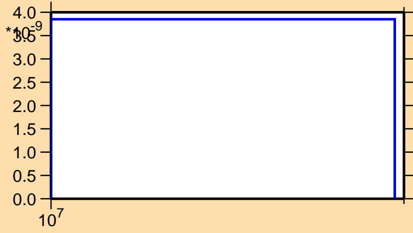
\sigma vs. E for ^{156}\text{Eu}(n,2n\alpha)
