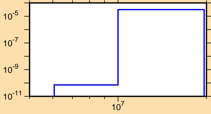
\sigma vs. E for ^{156}\text{Eu}(n,n\alpha)
