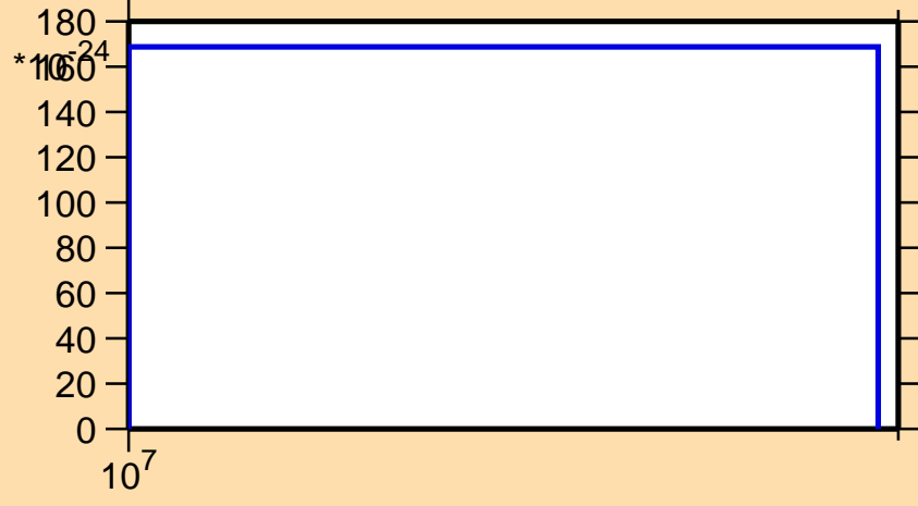
\sigma vs. E for ^{156}\text{Eu} (mt 11)
