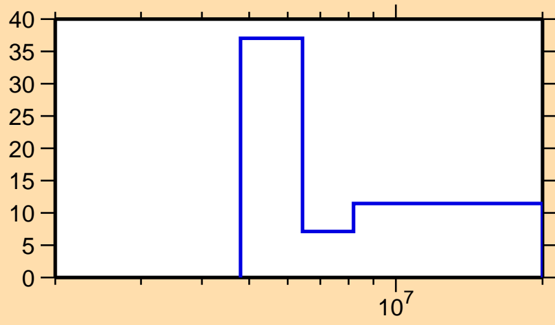
\Delta\sigma/\sigma vs. E for ^{156}\text{Eu}(n,2n)
