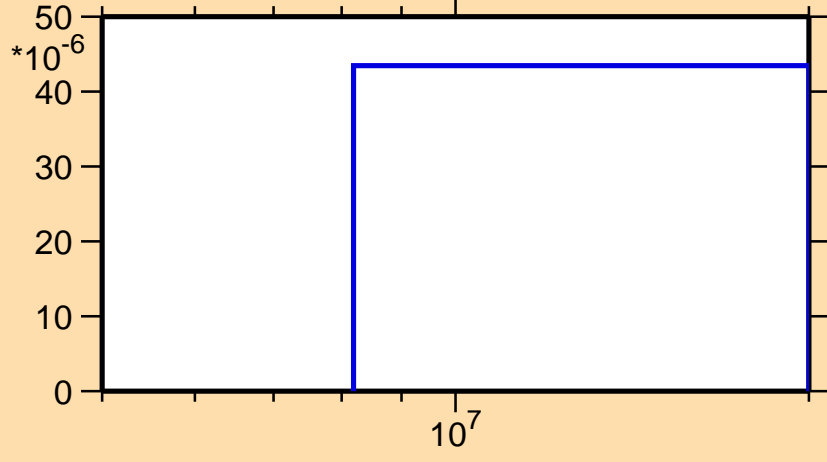
\sigma vs. E for ^{156}\text{Eu}(n,t)
