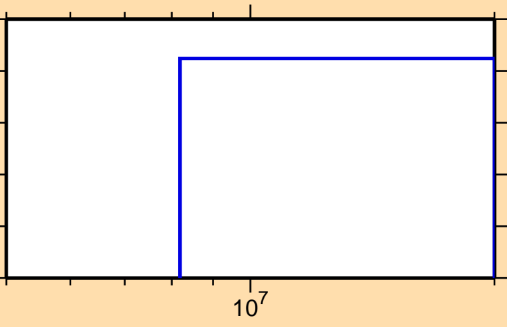
\sigma vs. E for ^{156}\text{Eu}(n,3n)
