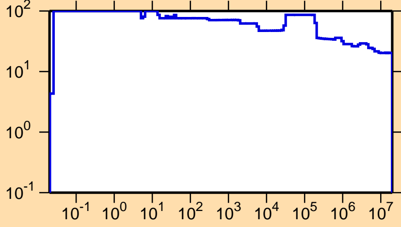
\Delta\sigma/\sigma vs. E for ^{158}\text{Eu}(n,\text{nonel.})
