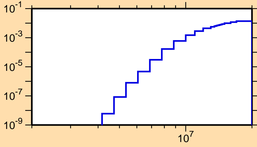
\sigma vs. E for ^{158}\text{Eu}(n,p)
