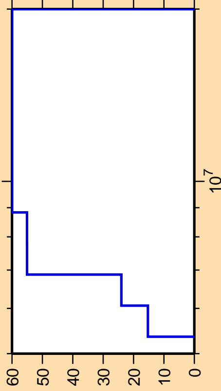
\Delta\sigma/\sigma vs. E for ^{160}\text{Eu}(n,n\text{cont.})
