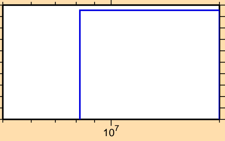
\sigma vs. E for ^{160}\text{Eu}(n,t)
