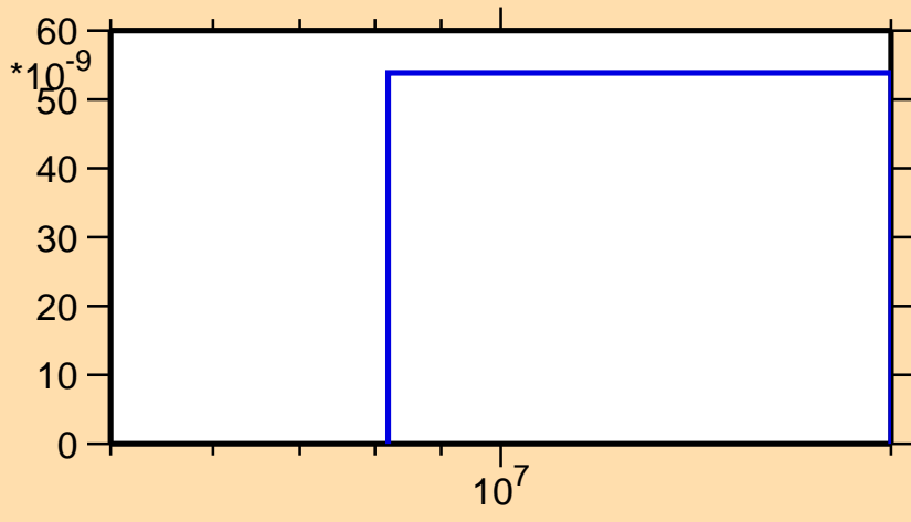
\sigma vs. E for ^{160}\text{Eu}(n,nd)
