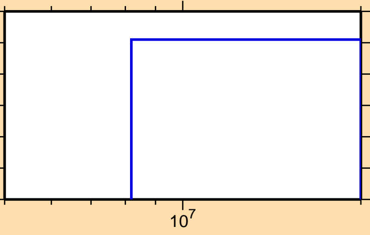
\sigma vs. E for ^{160}\text{Eu}(n,np)
