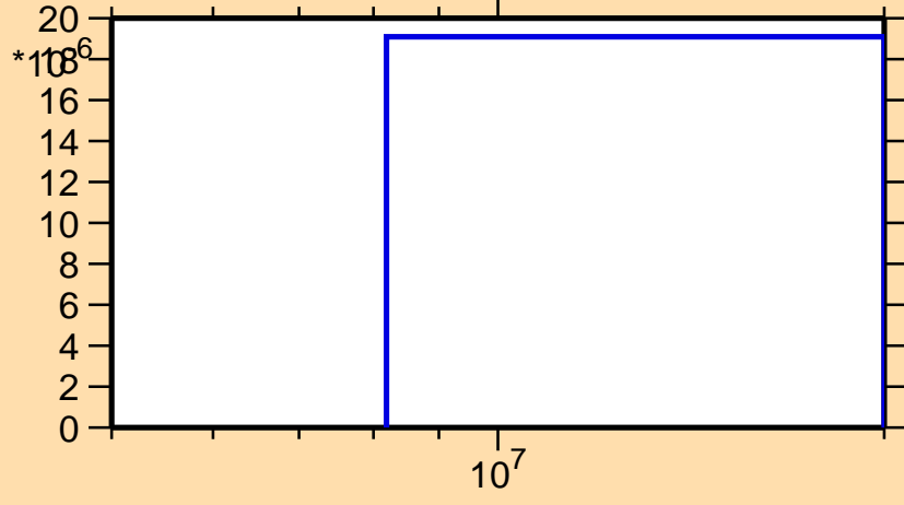
\sigma vs. E for ^{160}\text{Eu}(n,t)
