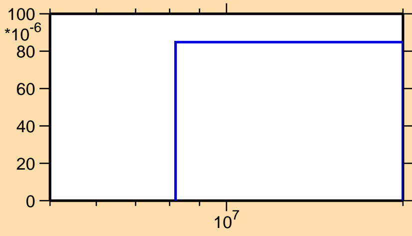
\sigma vs. E for ^{160}\text{Eu}(n,d)
