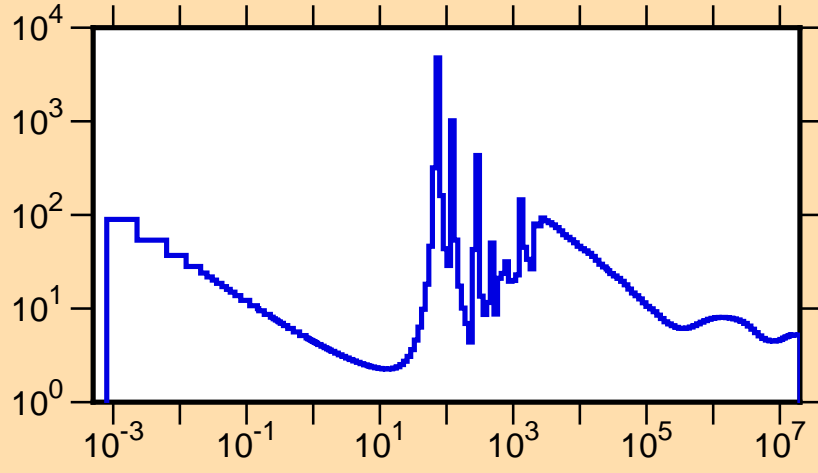
\sigma vs. E for ^{161}\text{Eu}(n,\text{tot.})
