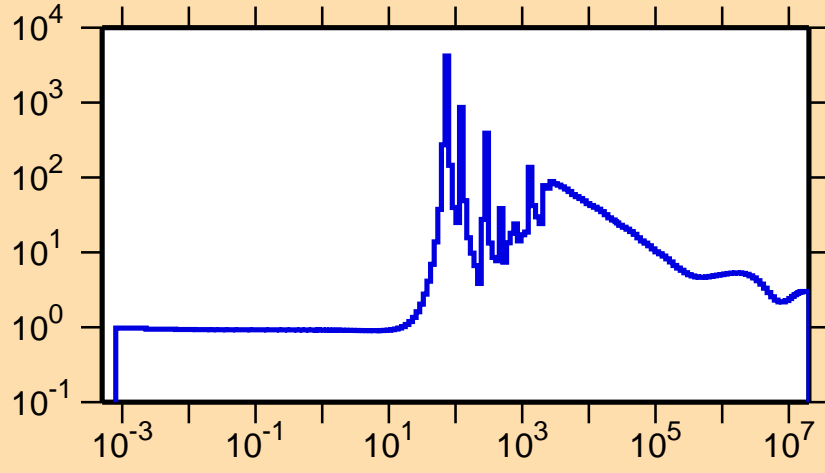
\sigma vs. E for ^{161}\text{Eu}(n,\text{el.})
