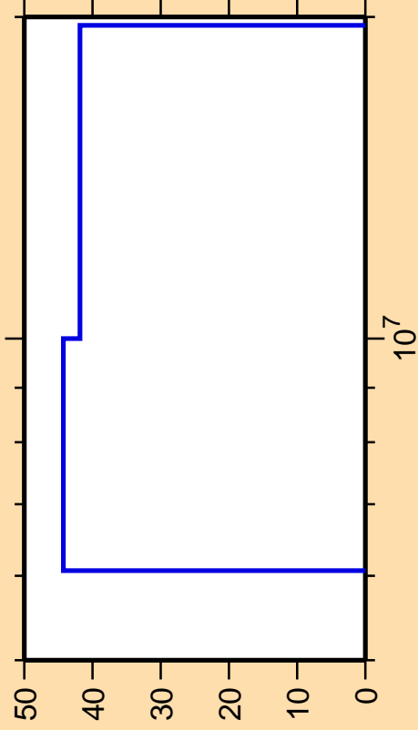
\Delta\sigma/\sigma vs. E for ^{161}\text{Eu}(n,n_1)
