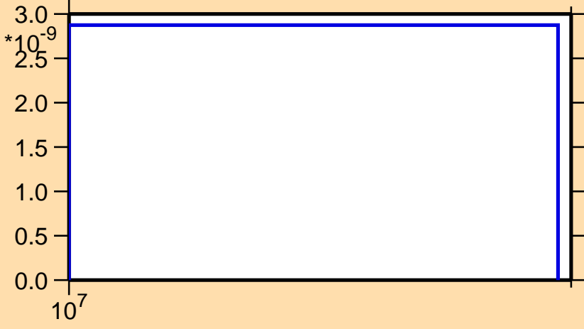
\sigma vs. E for ^{161}\text{Eu}(n,\text{nd})
