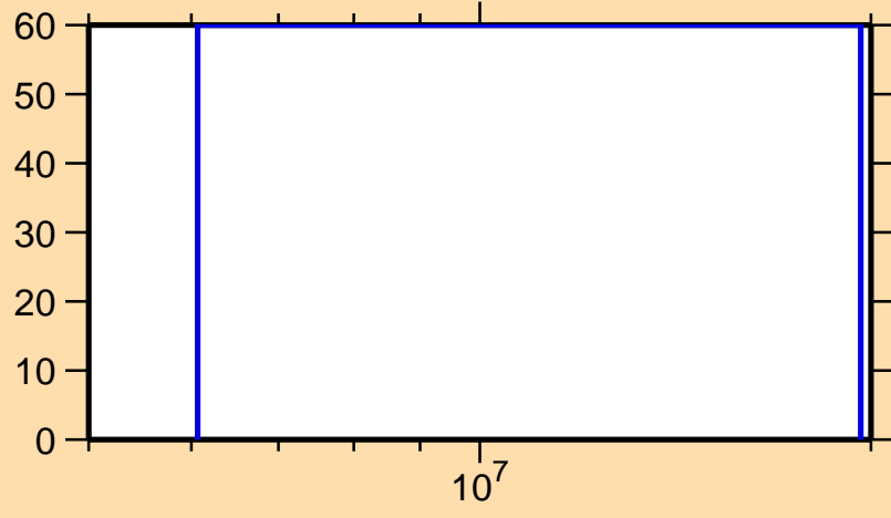
\Delta\sigma/\sigma vs. E for ^{161}\text{Eu}(n,n\text{cont.})
