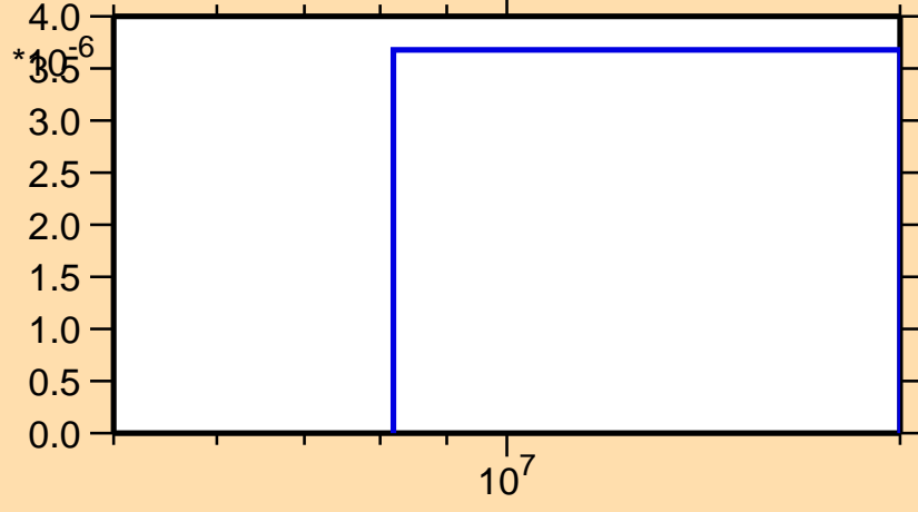
\sigma vs. E for ^{161}\text{Eu}(n,n\alpha)
