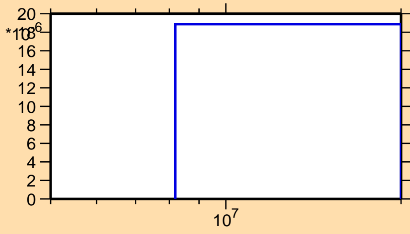
\sigma vs. E for ^{162}\text{Eu}(n,np)
