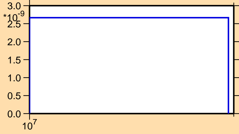
\sigma vs. E for ^{163}\text{Eu}(n,\text{nd})
