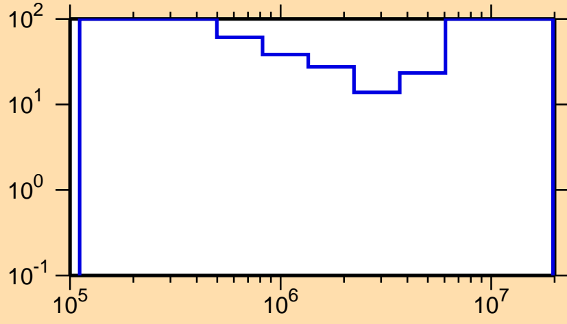
\Delta\sigma/\sigma vs. E for ^{163}\text{Eu}(n,n\text{cont.})
