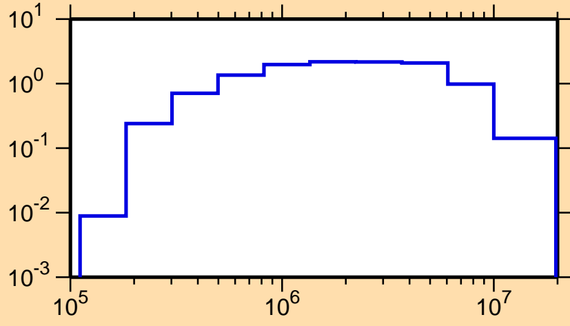
\sigma vs. E for ^{163}\text{Eu}(n,n\text{cont.})
