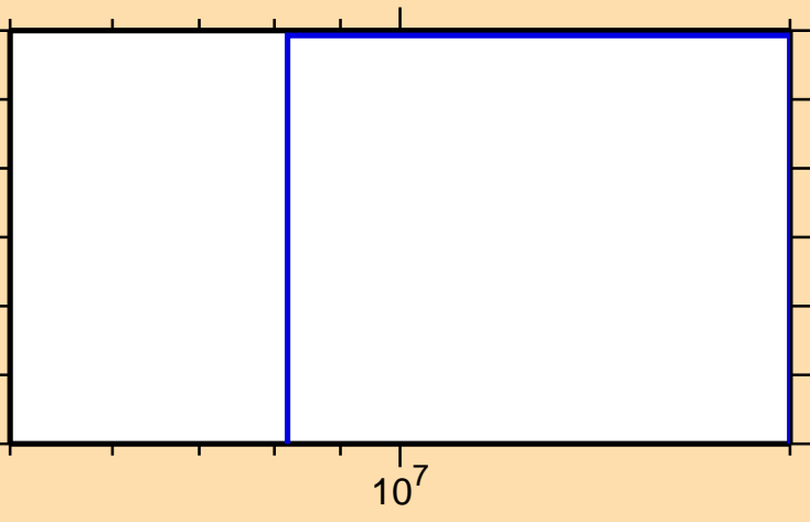
\sigma vs. E for ^{163}\text{Eu}(n,d)
