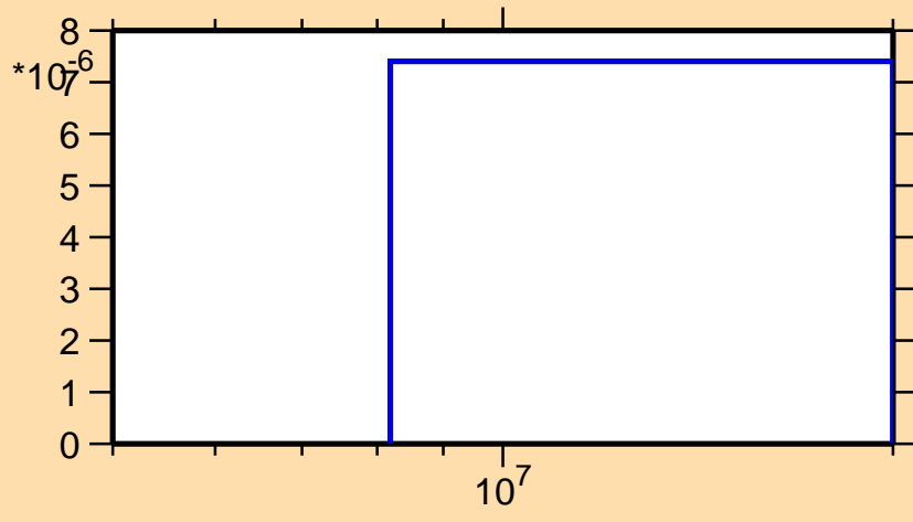
\sigma vs. E for ^{163}\text{Eu}(n,t)
