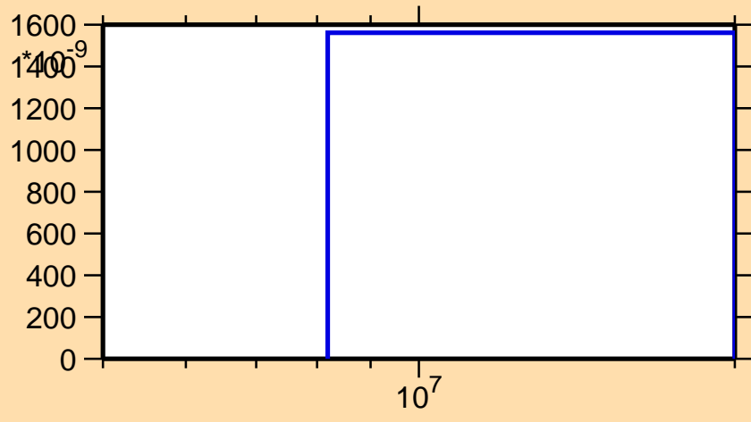
\sigma vs. E for ^{163}\text{Eu}(n,n\alpha)
