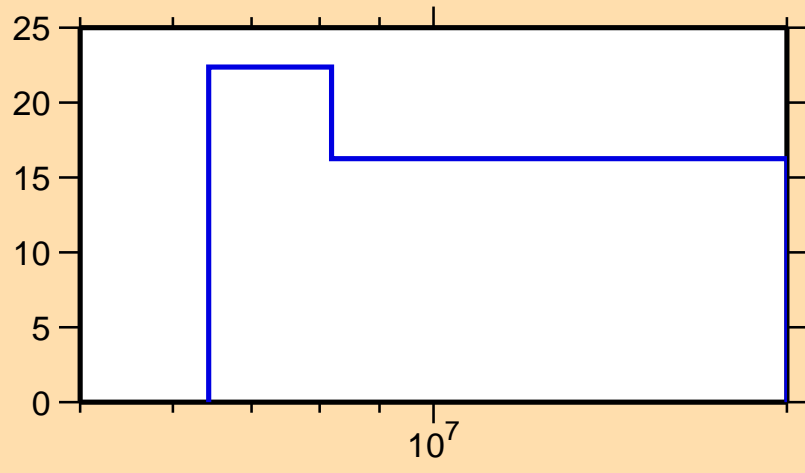
\Delta\sigma/\sigma vs. E for ^{163}\text{Eu}(n,el.)
