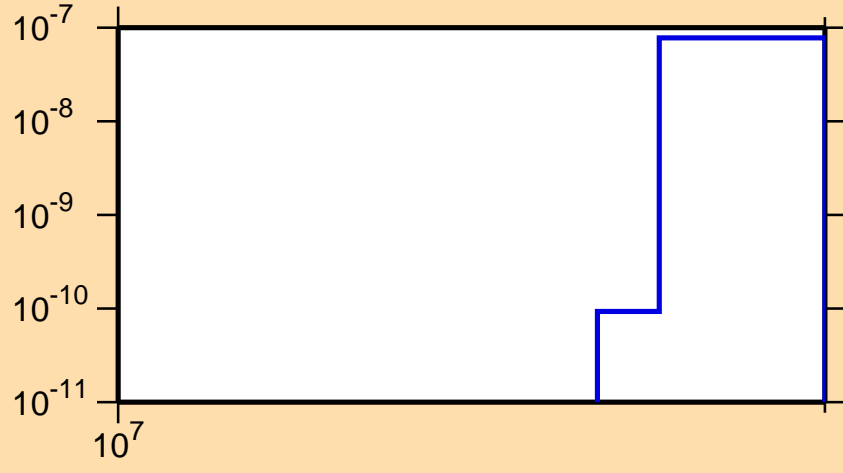
\sigma vs. E for ^{164}\text{Eu}(n,2np)
