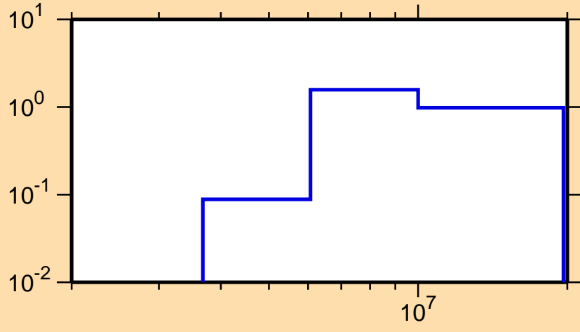
\sigma vs. E for ^{164}\text{Eu}(n,2n)
