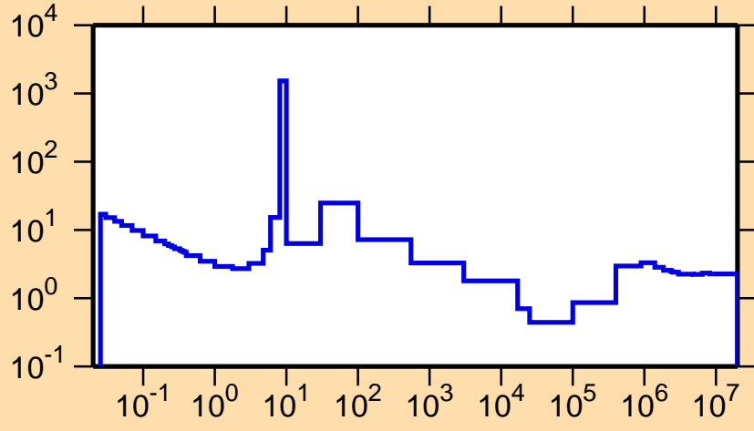
\sigma vs. E for ^{164}\text{Eu}(n,\text{nonel.})
