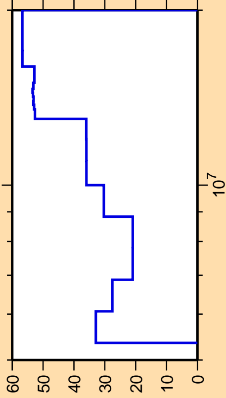
\Delta\sigma/\sigma vs. E for ^{165}\text{Eu}(n,2n)
