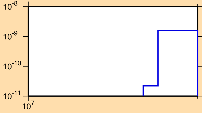
\sigma vs. E for ^{165}\text{Eu}(n,2n\alpha)
