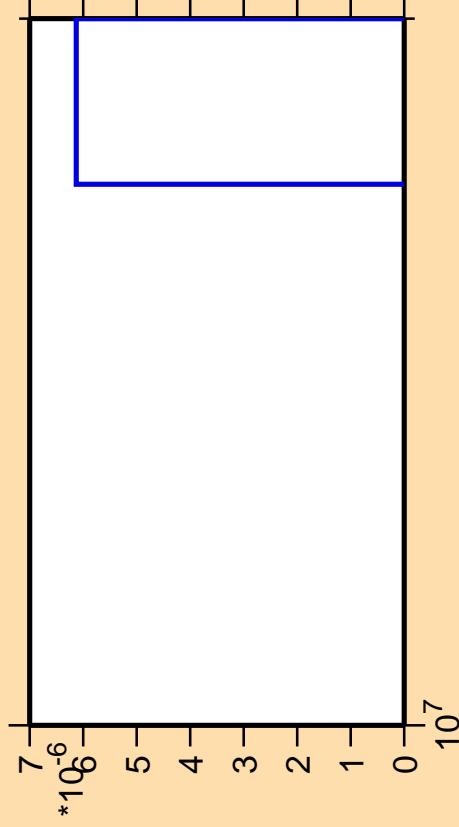
\Delta\sigma/\sigma vs. E for ^{165}\text{Eu} (mt 42)
