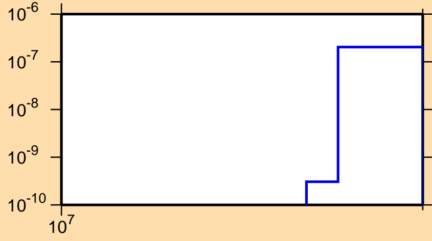
\sigma vs. E for ^{165}\text{Eu}(n,\text{nd})
