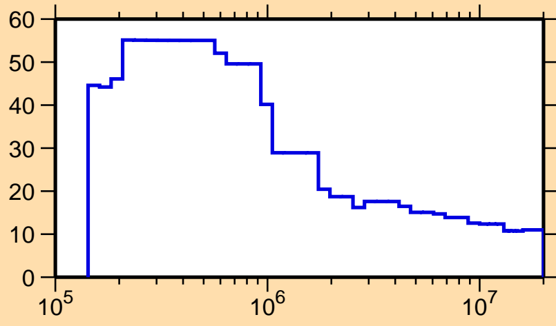
\Delta\sigma/\sigma vs. E for ^{165}\text{Eu}(n,\text{nonel.})
