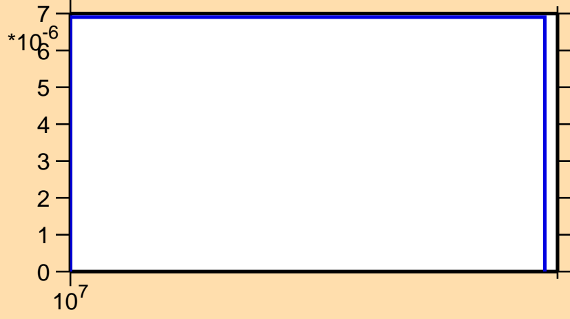
\sigma vs. E for ^{165}\text{Eu}(n,np)
