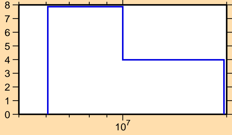
\Delta\sigma/\sigma vs. E for ^{165}\text{Eu}(n,\text{tot.})
