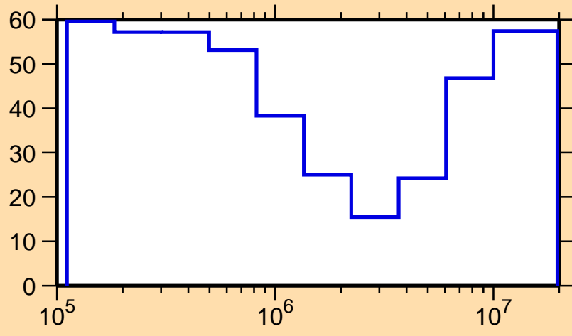
\Delta\sigma/\sigma vs. E for ^{165}\text{Eu}(n,\text{inel.})
