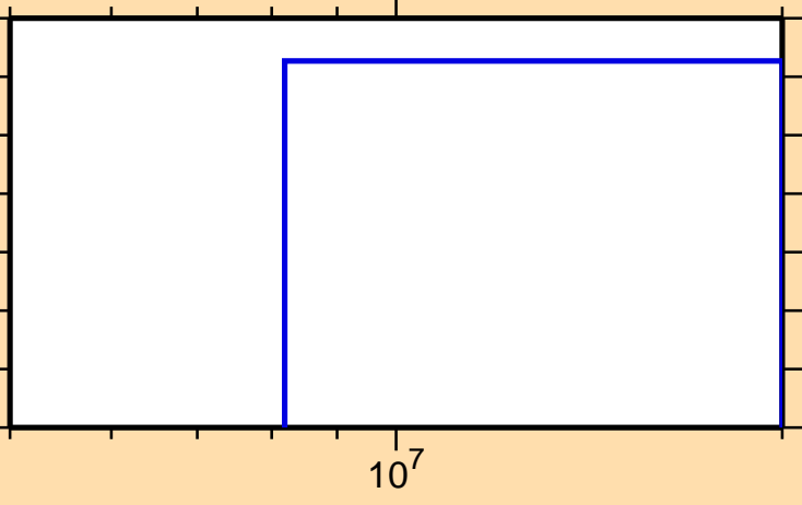
\sigma vs. E for ^{165}\text{Eu}(n,d)
