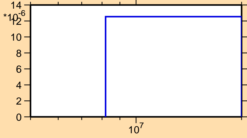
\sigma vs. E for ^{165}\text{Eu}(n,d)
