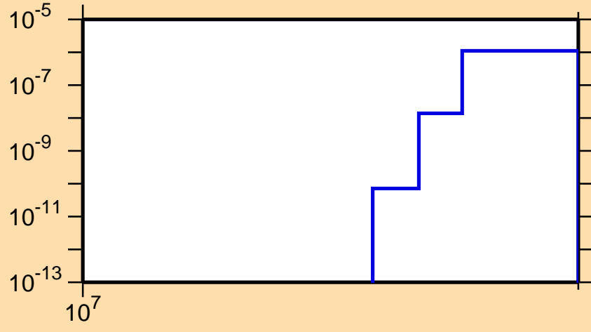
\sigma vs. E for ^{166}\text{Eu}(n,nd)
