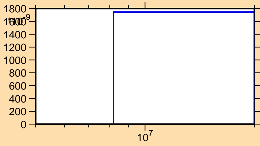
\sigma vs. E for ^{166}\text{Eu}(n,np)
