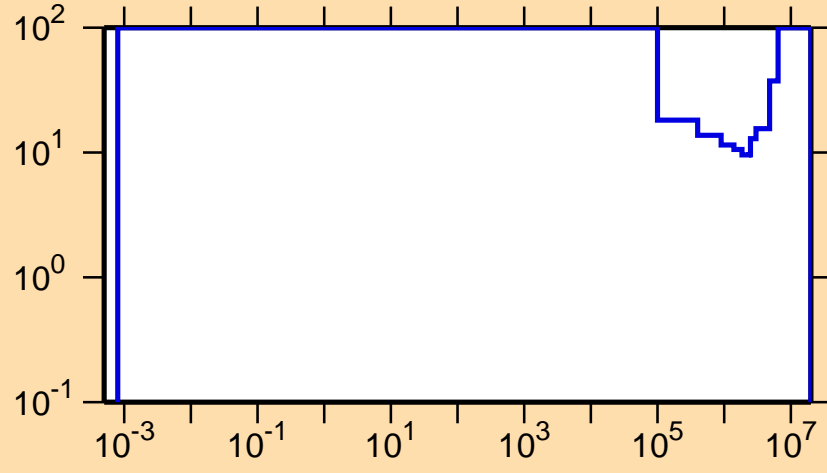
\Delta\sigma/\sigma vs. E for ^{17}\text{F}(n,p)
