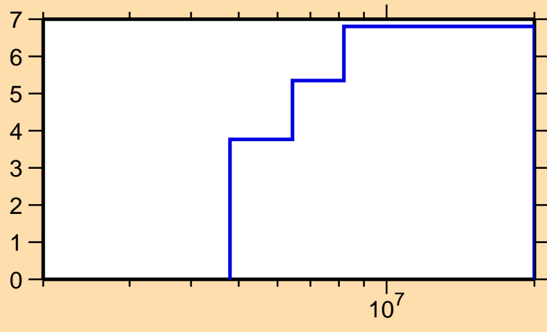
\Delta\sigma/\sigma vs. E for ^{17}\text{F}(n,\text{nonel.})
