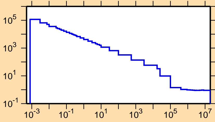
\sigma vs. E for ^{17}\text{F}(n,\text{nonel.})
