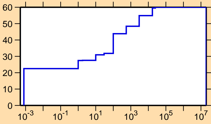
\Delta\sigma/\sigma vs. E for ^{17}\text{F}(n,\gamma)
