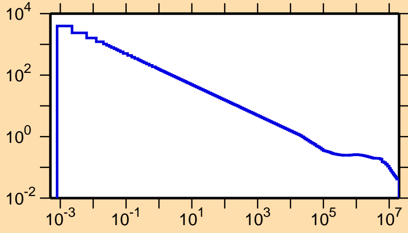
\sigma vs. E for ^{18}\text{F}(n,p)
