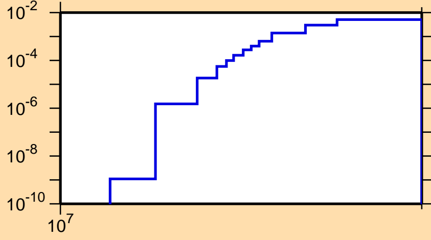
\sigma vs. E for ^{18}\text{F}(\text{mt117})
