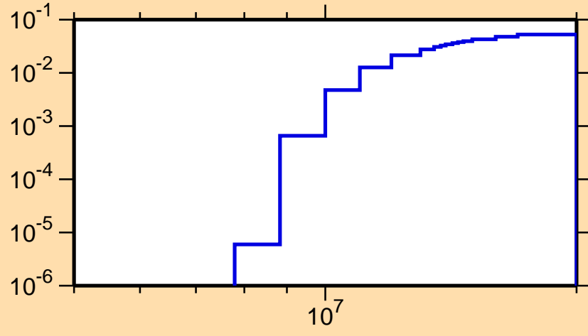
\sigma vs. E for ^{18}\text{F}(n,\text{nd})
