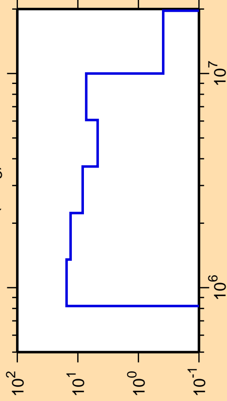
\Delta\sigma/\sigma vs. E for ^{18}\text{F}(n,n_3)
