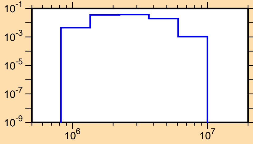
\sigma vs. E for ^{18}\text{F}(n,n_3)
